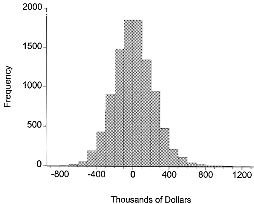
Figure 1. Four Week Value-at-Risk Example
